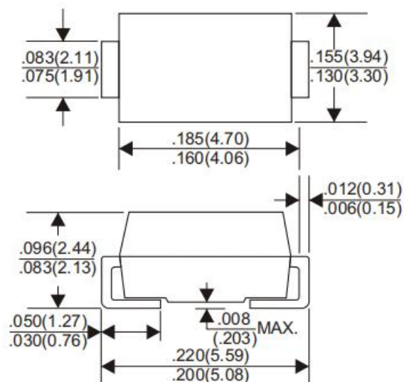
DO-214AA(SMB)
