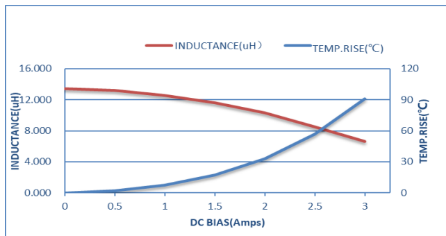
ZETC322520S150MBT-LF
