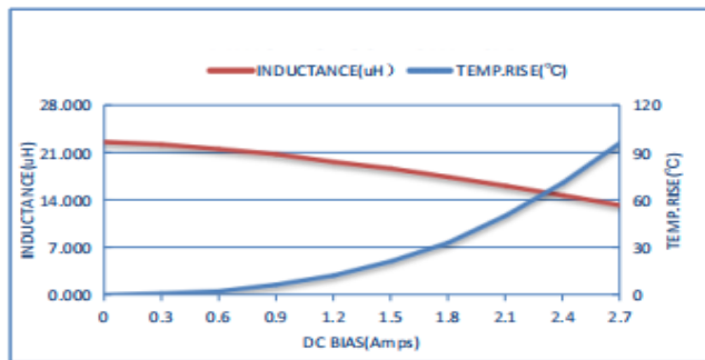
ZETC322520S220MBT-LF
