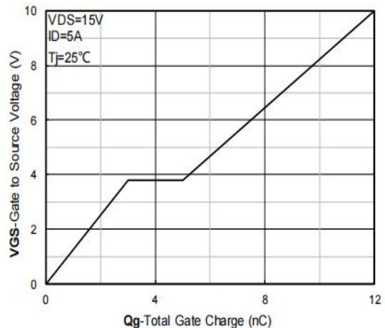
Figure 6: Gate-Charge Characteristics
