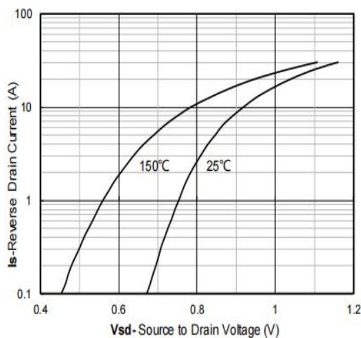
Figure 9: Diode Characteristics
