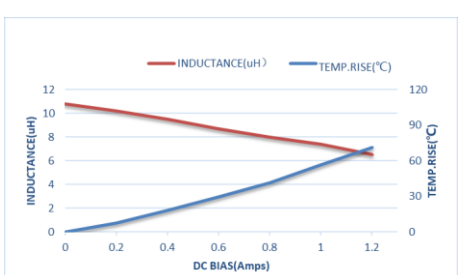
ZEMS201610-100M
