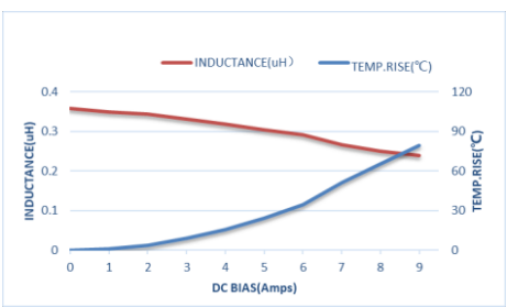
ZEMS201610-R33M
