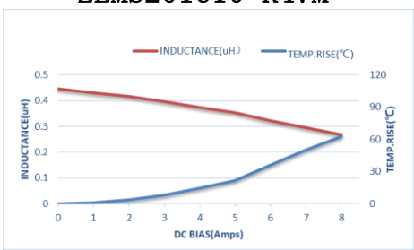
ZEMS201610-R47M
