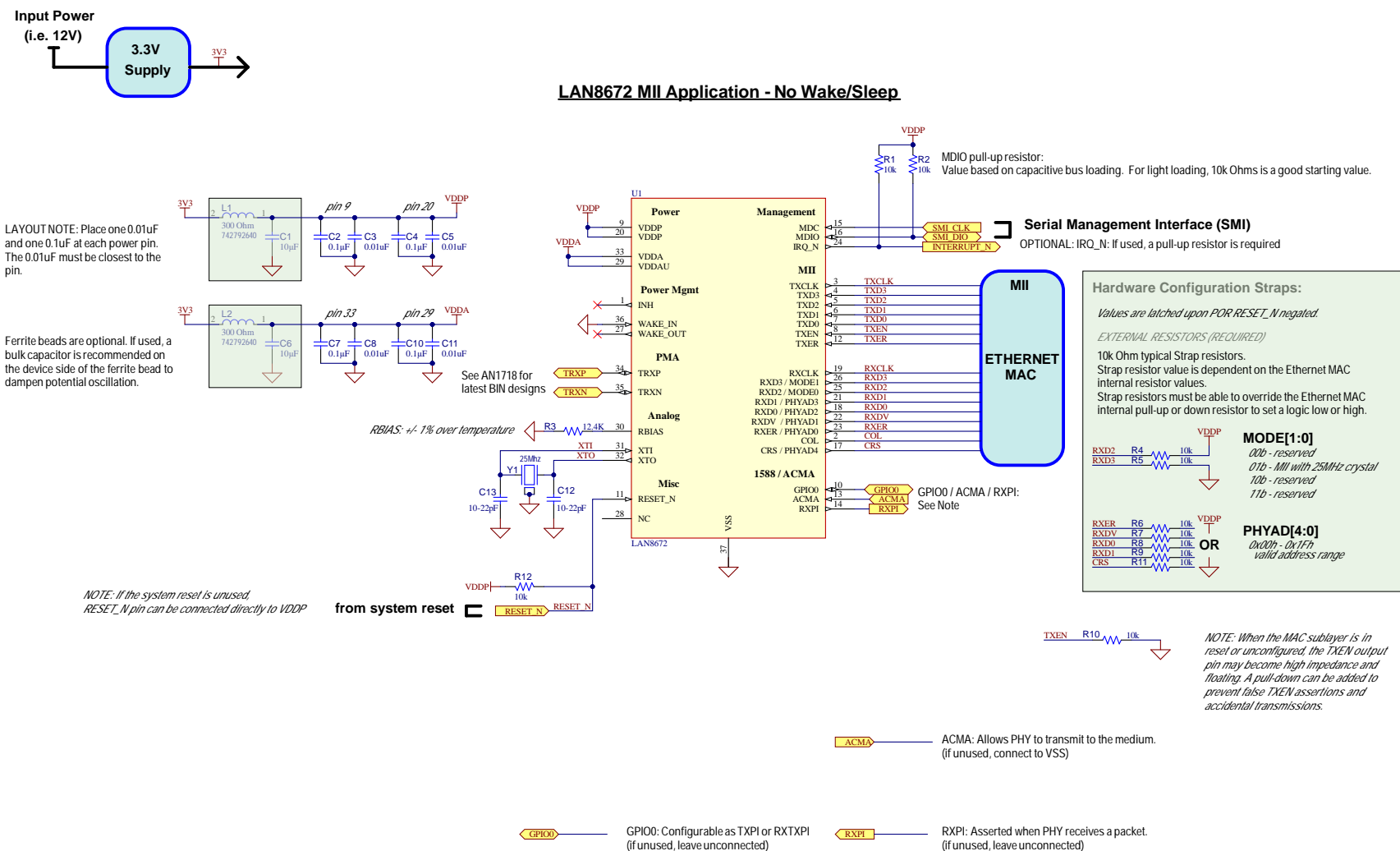
Figure 6-17. LAN8672 MII Reference Schematic (No Sleep/Wake)
