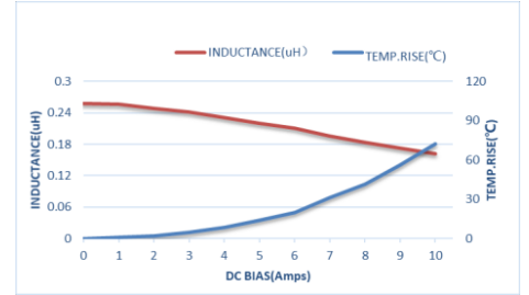
ZEMS201610-R22M
