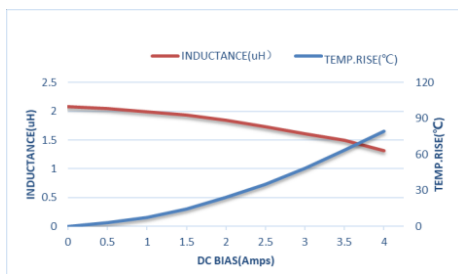
ZEMS201610-2R2M
