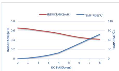
ZEMS201610-R68M
