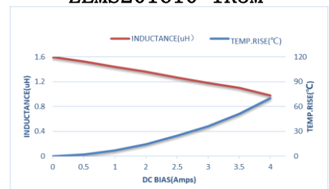
ZEMS201610-1R5M
