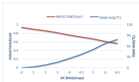
ZEMS201610-1R0M
