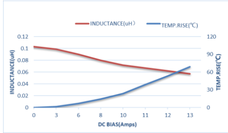
ZEMS201610-R10M
