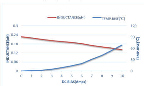
ZEMS201610-R24M
