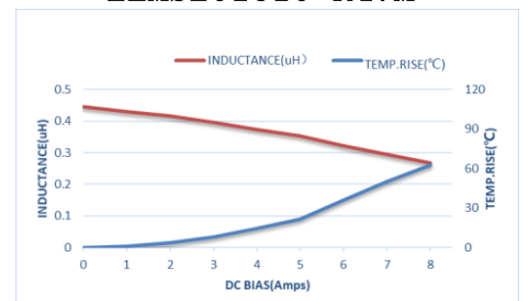
ZEMS201610-R47M
