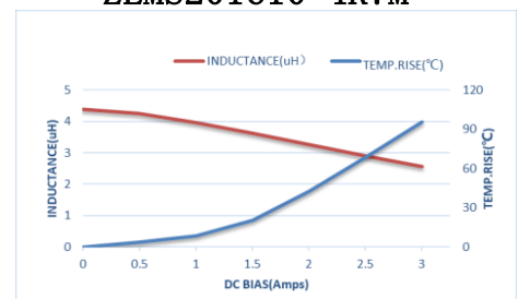
ZEMS201610-4R7M
