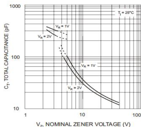
Figure 4: Capacitance Characteristics
