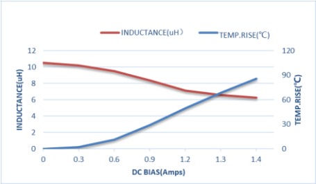
ZEP IM201608T100MLF
