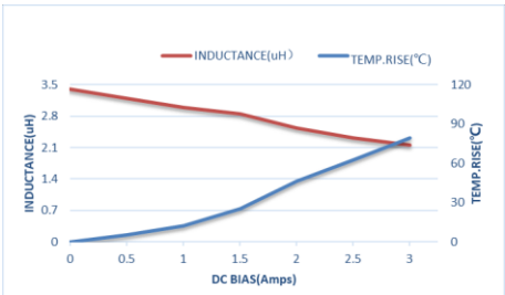
ZEP IM201608T3R3MLF
