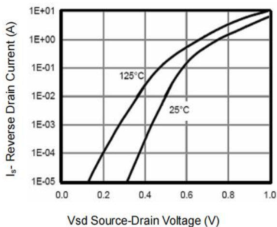
Figure 7: Diode Characteristics
