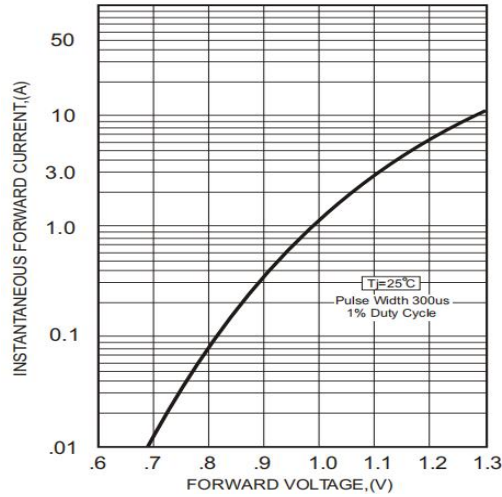
Figure 1: Forward Characteristics
