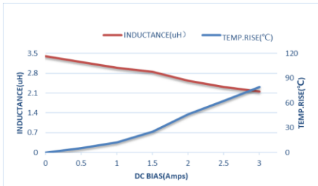
ZETC201608S-3R3MT-LF
