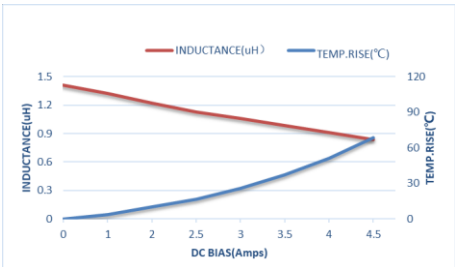
ZETC201608S-1R5MT-LF
