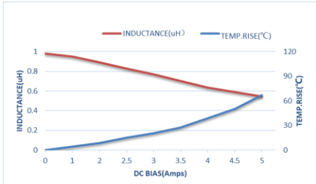
ZETC201608S-1R0MT-LF
