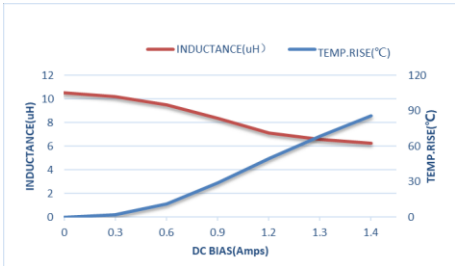
ZETC201608S-100MT-LF
