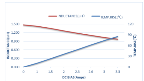
ZEPIM201208S-1R5M
