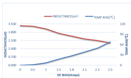
ZEPIM201208S-3R3M
