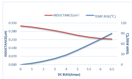
ZEPIM201208S-R33M
