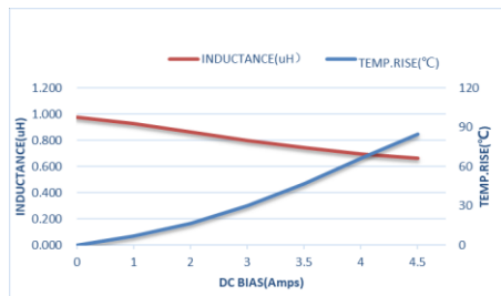
ZEPIM201208S-1R0M
