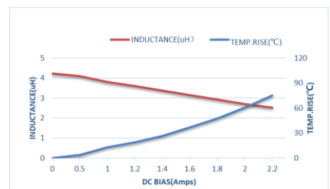
ZEPIM201208S-4R7M
