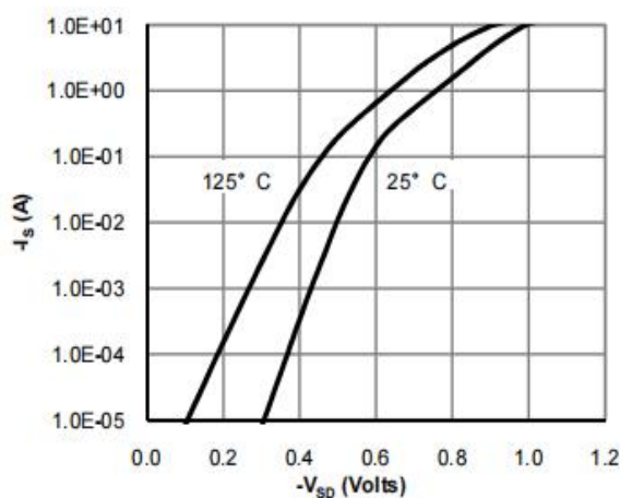
Figure 7: Diode Characteristics
