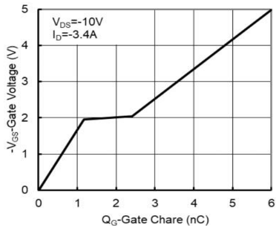
Figure 6: Gate-Charge Characteristics
