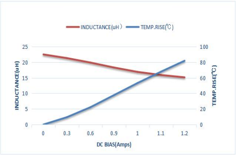
ZETC252010S-220MT-LF
