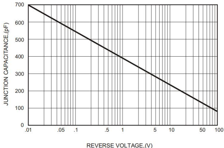
FIG.4-TYPICAL JUNCTION CAPACITANCE
