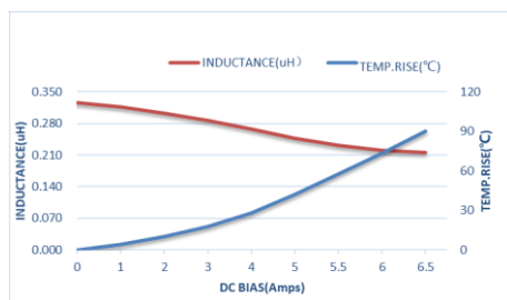
ZETC201208SR33MBT-LF
