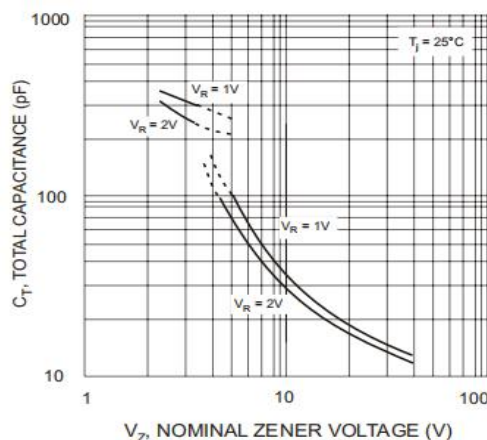
Figure 4: CA-6AF capacitance Characteristics
