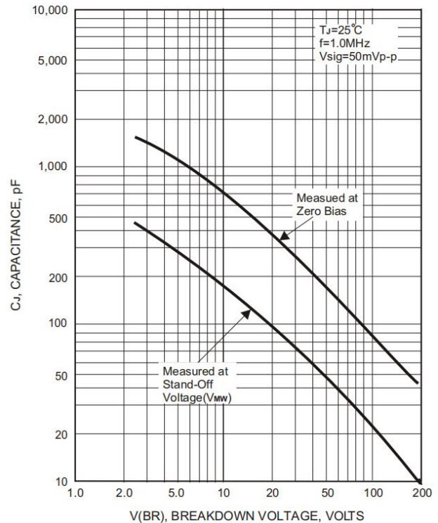
FIG.4-TYPICAL JUNCTION CAPACITANCE
