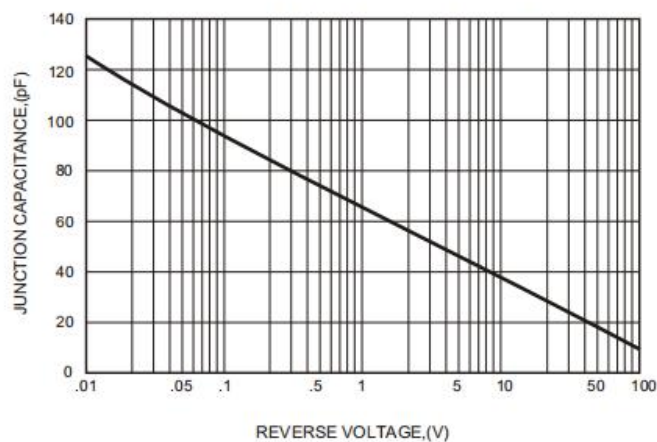
FIG.5-TYPICAL JUNCTION CAPACITANCE
