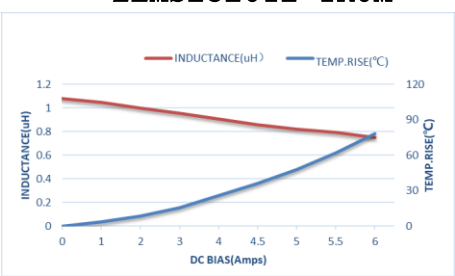
ZEMS252012-1R0M
