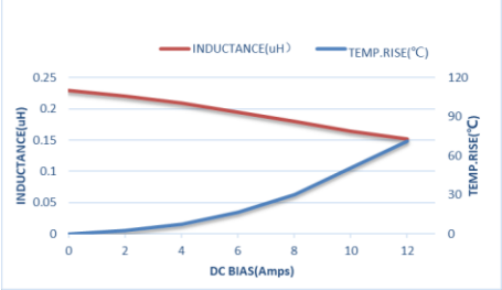
ZEMS252012-R22M
