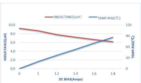
ZEMS252012-100M
