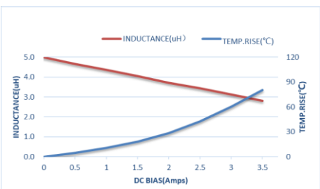
ZEMS252012-4R7M
