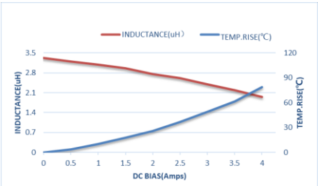
ZEMS252012-3R3M
