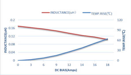
ZEMS252012-R15M
