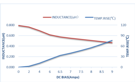
ZEMS252012-R82M
