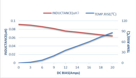
ZEMS252012-R10M
