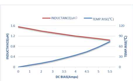
ZEMS252012-1R5M
