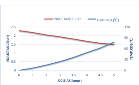
ZEMS252012-2R2M
