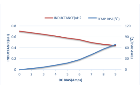
ZEMS252012-R68M
