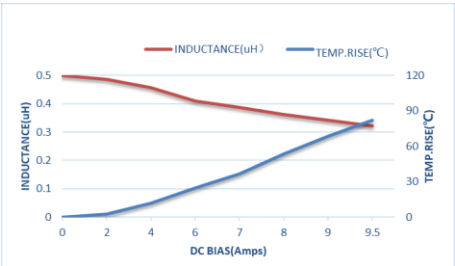
ZEMS252012-R47M
