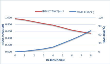
ZEPIM252010S-1R0M
