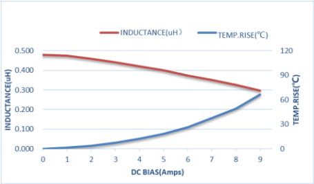
ZEPIM252010S-R47M
