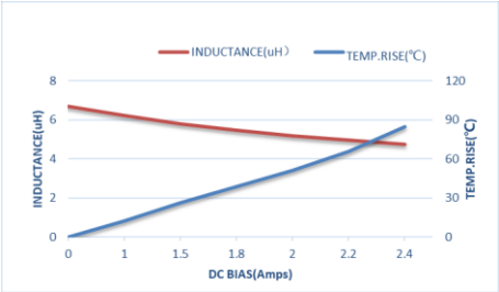
ZEPIM252010S-6R8M
