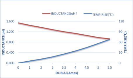
ZEPIM252010S-1R5M
