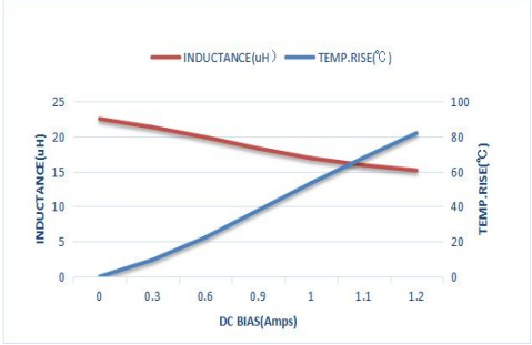
ZEPIM252010S-220M
