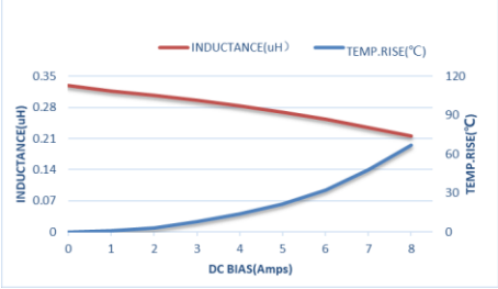
ZEPIM252010S-R33M
