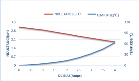
ZEPIM252010S-3R3M
