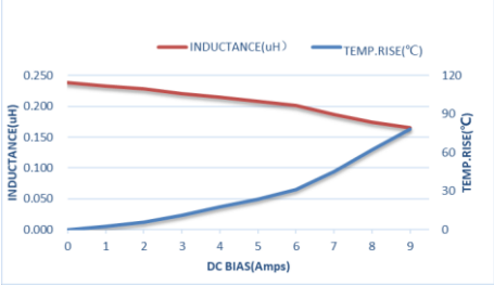
ZEPIM252010S-R24M
