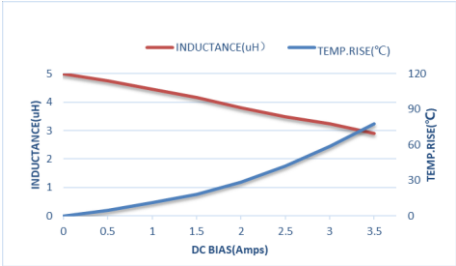
ZEPIM252010S-4R7M
