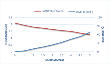
ZEPIM252010S-2R2M
