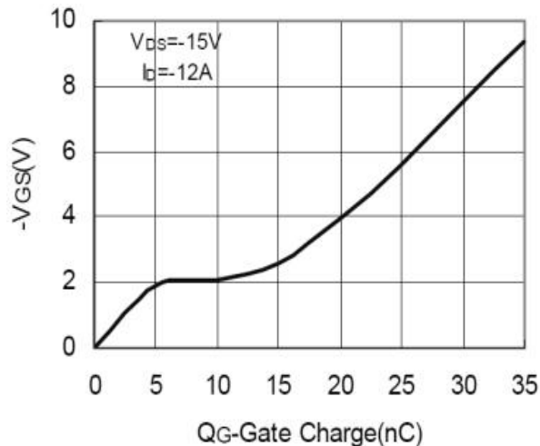
Figure 6: Gate-Charge Characteristics
