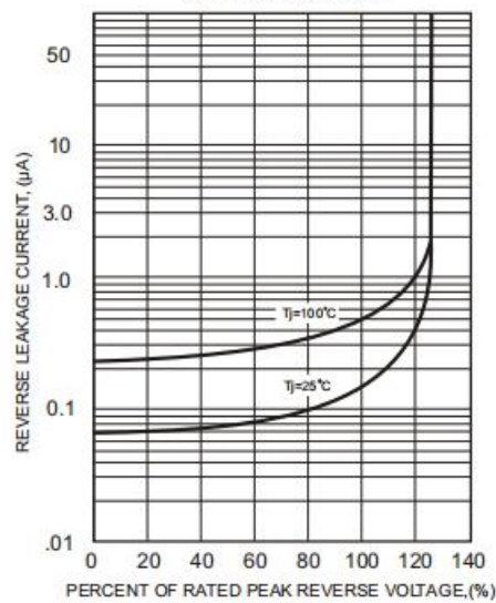
FIG.4-TYPICAL REVERSE CHARACTERISTICS
