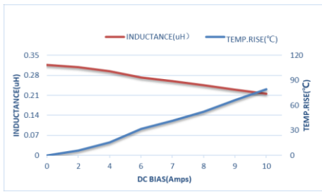
ZETC252012SR33MBT-LF
