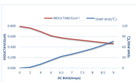
ZETC252012SR82MBT-LF
