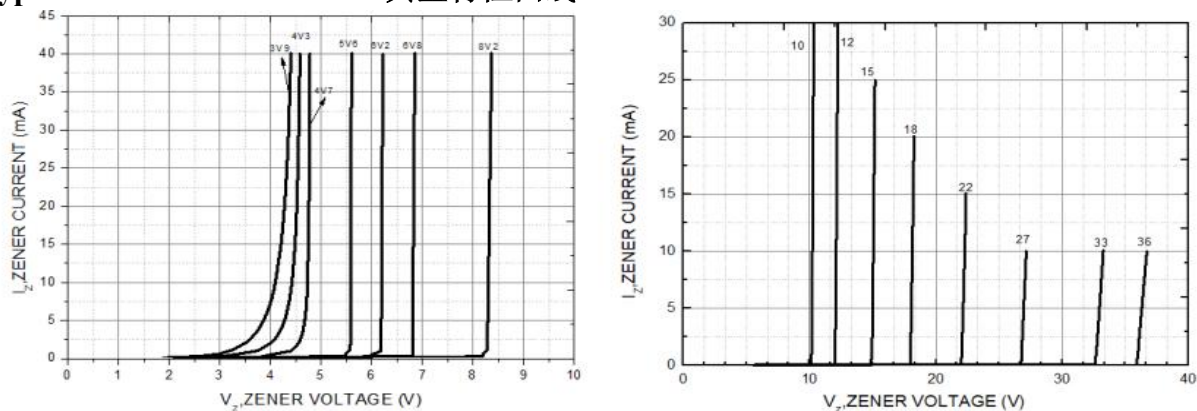
Figure 1: Zener Characteristics
