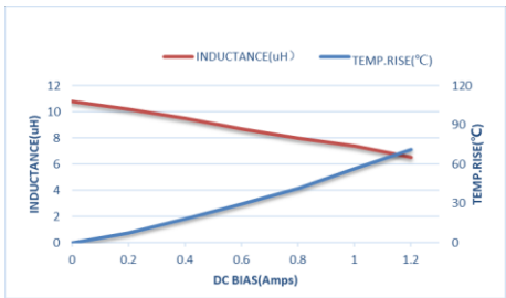
ZET-CORE-201610ST100MBCA
