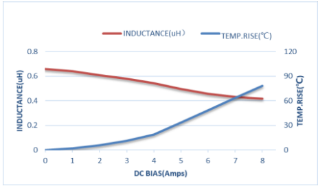
ZET-CORE-201610STR68MBCA
