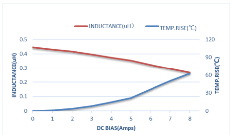
ZET-CORE-201610STR47MBCA
