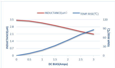
ZET-CORE-201610ST3R3MBCA
