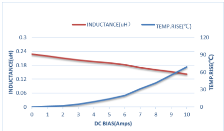
ZET-CORE-201610STR24MBCA
