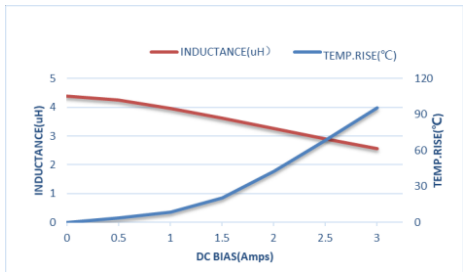
ZET-CORE-201610ST4R7MBCA
