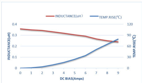
ZET-CORE-201610STR33MBCA
