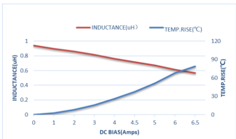
ZET-CORE-201610ST1R0MBCA
