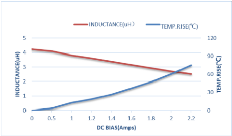
ZEMS201208-4R7M
