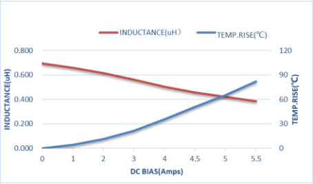
ZEMS201208-R68M
