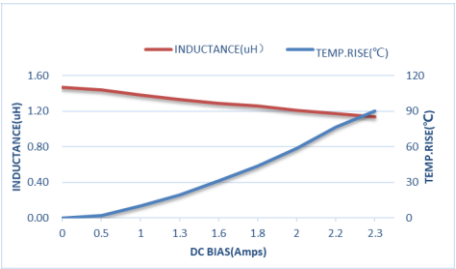
ZETC160808S1R5MBT-LF
