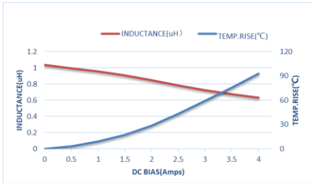
ZETC160808S1R0MBT-LF
