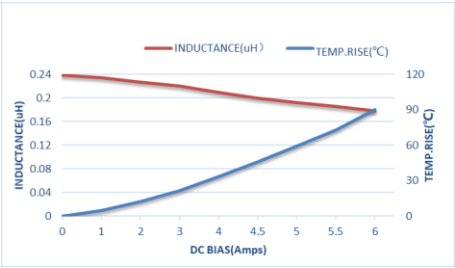
ZETC160808SR24MBT-LF
