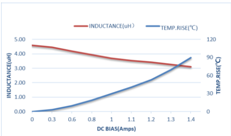
ZETC160808S4R7MBT-LF
