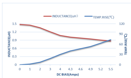
ZEPIM252008S-1R5M
