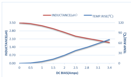
ZEPIM252008S-3R3M
