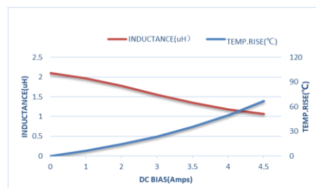
ZEPIM252008S-2R2M
