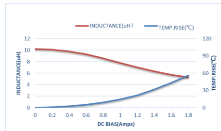
ZEPIM252008S-100M
