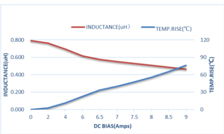
ZETC252012SR82MBT-LF
