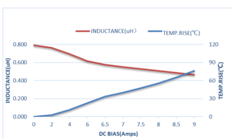
ZEPIM252012S-R82M
