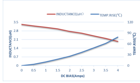
ZEPIM252012S-3R3M
