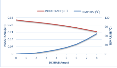
ZEPIM252010TR33MLF
