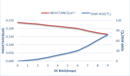
ZEPIM252010TR22MLF
