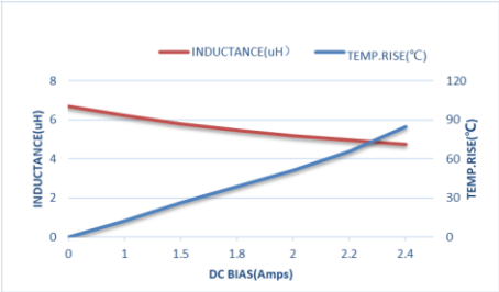
ZEPIM252010T6R8MLF
