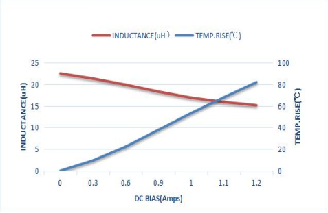
ZEPIM252010T220MLF
