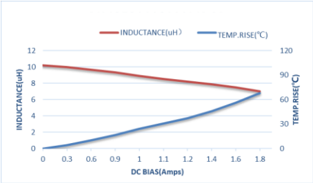
ZEPIM252010T100MLF
