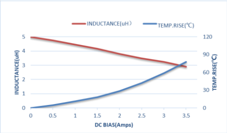
ZEPIM252010T4R7MLF
