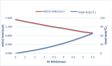
ZEPIM252010T1R5MLF
