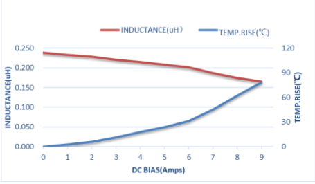
ZEPIM252010TR24MLF
