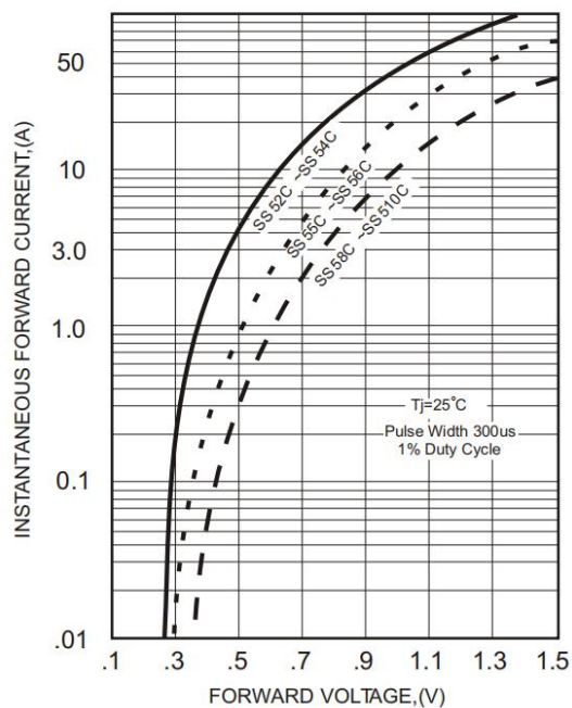
FIG.2-TYPICAL FORWARD CHARACTERISTICS
