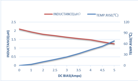
ZETC252010S2R2MBT-LF
