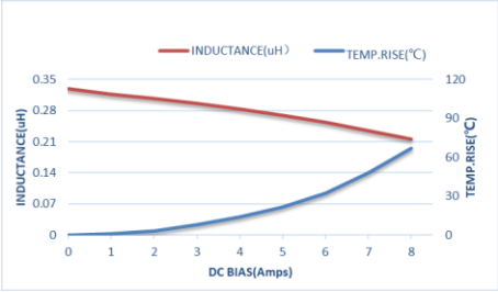
ZETC252010SR33MBT-LF
