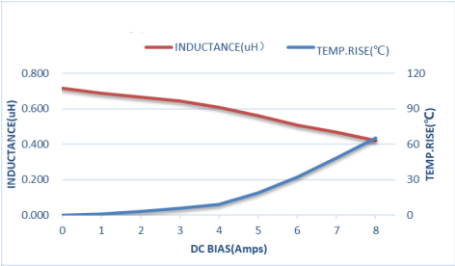
ZETC252010SR68MBT-LF
