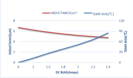
ZETC252010S6R8MBT-LF
