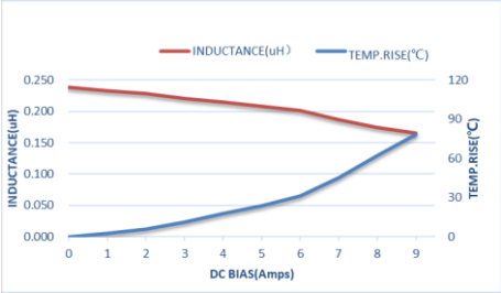
ZETC252010SR24MBT-LF
