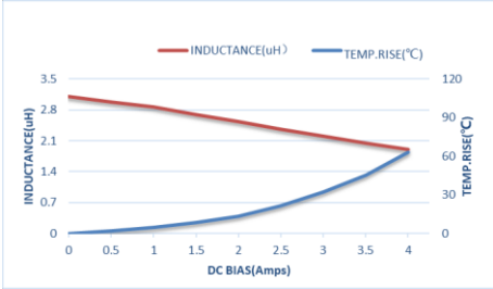
ZETC252010S3R3MBT-LF
