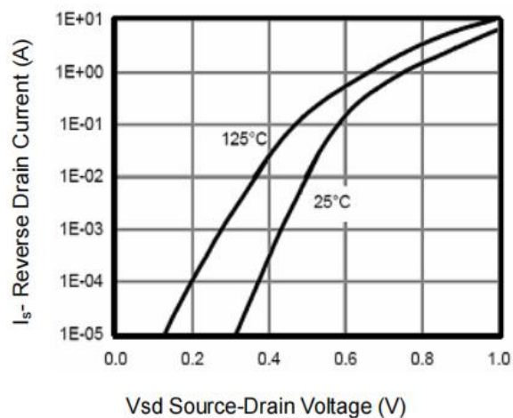
Figure 7: Diode Characteristics
