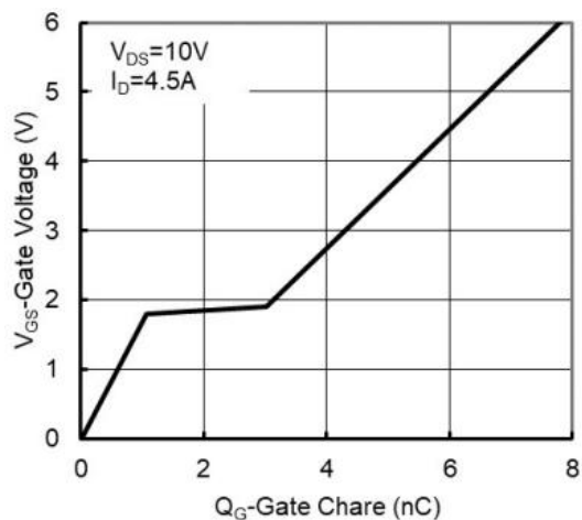
Figure 6: Gate-Charge Characteristics
