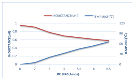
ZETC201612S-1R0MT-LF
