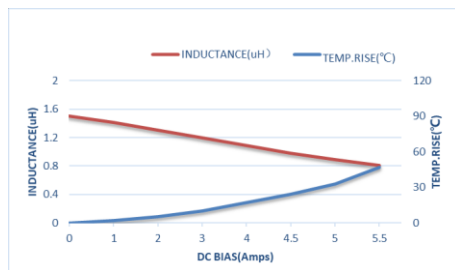
ZETC201612S-1R5MT-LF
