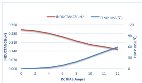
ZETC201612S-R33MT-LF
