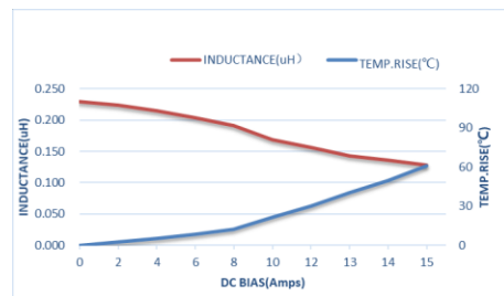
ZETC201612S-R24MT-LF
