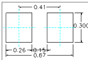
Soldering Pattern
