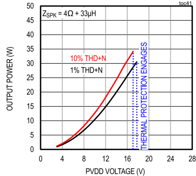
OUTPUT POWER vs. PVDD SUPPLY VOLTAGE
