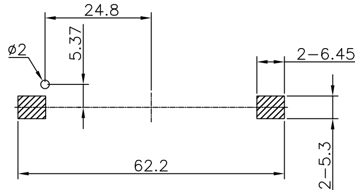
PCB Layout Diagram TOP View
