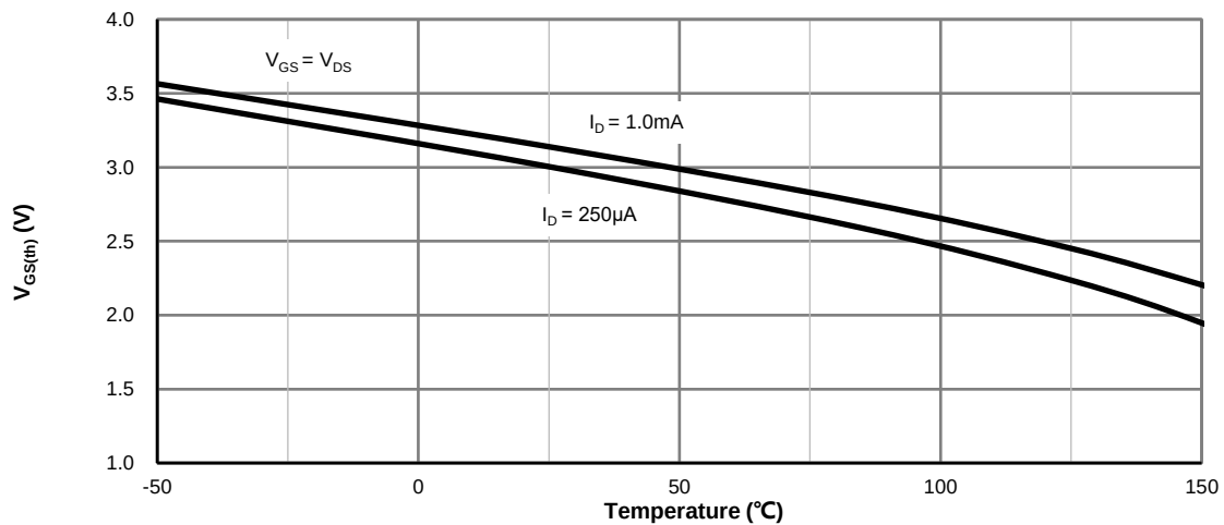
Figure 5: V_{GS(th)} vs. Junction Temperature
