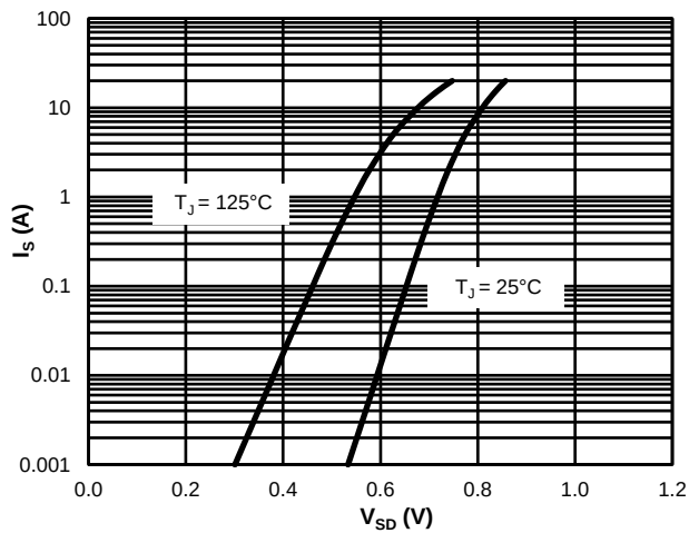
Figure 7: Body-Diode Characteristics
