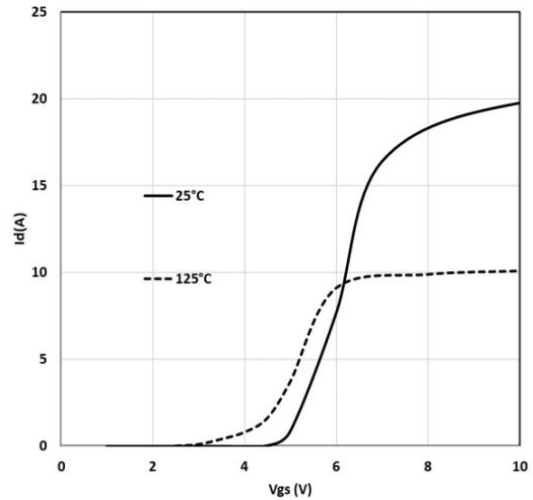
Fig.2 Transfer characteristics
