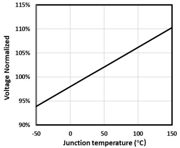
Fig.8 Drain-Source Breakdown Voltage
