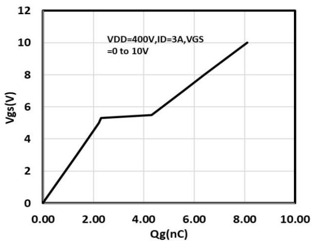
Fig.5 Gate charge
