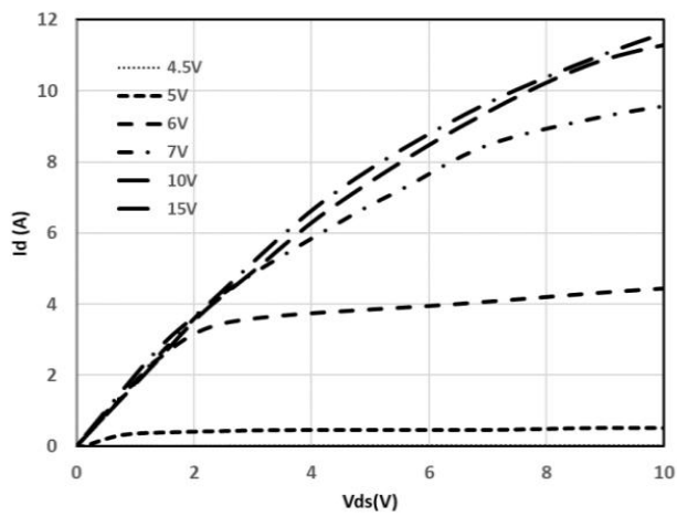
Fig.1 Typical Output characteristics ( 25^{\circ}\text{C} )
