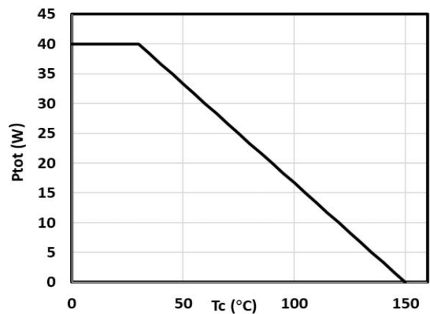
Fig.4 Power dissipation
