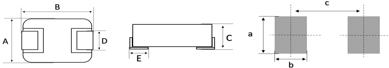
封裝尺寸 (mm) Dimension
