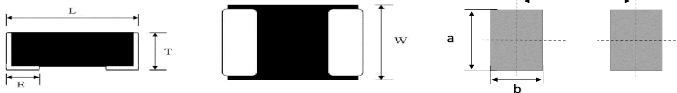
封裝尺寸 Dimension (mm)
