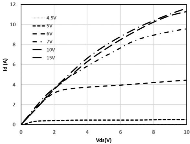
Fig.1 Typical Output characteristics ( 25^{\circ}\text{C} )
