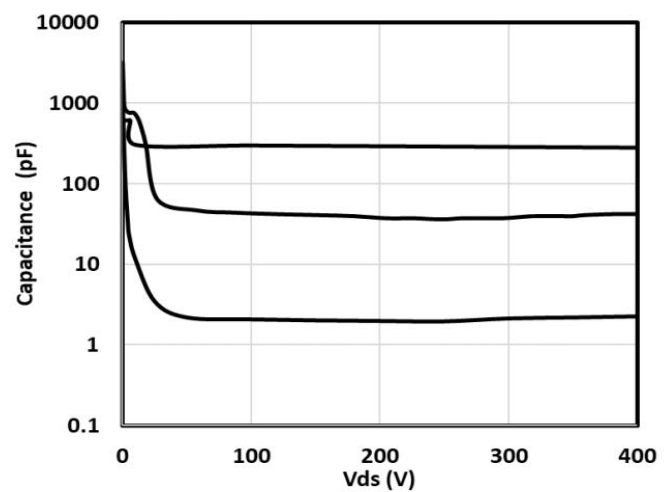
Fig.6 Typical capacitance characteristics
