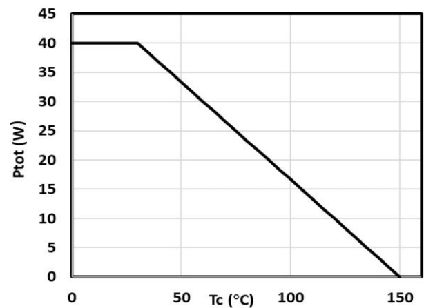
Fig.4 Power dissipation
