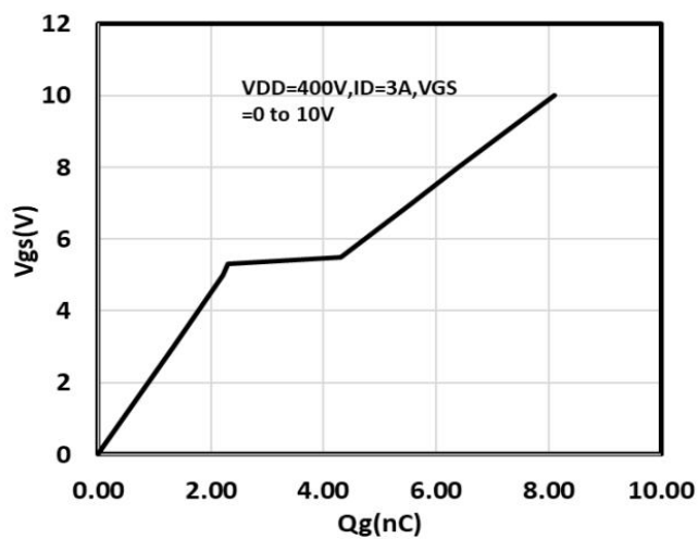
Fig.5 Gate charge
