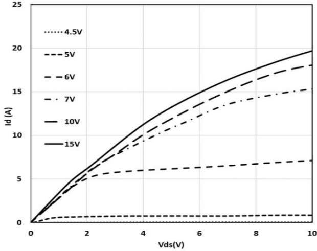
Fig.1 Typical Output characteristics ( 25^{\circ}\text{C} )
