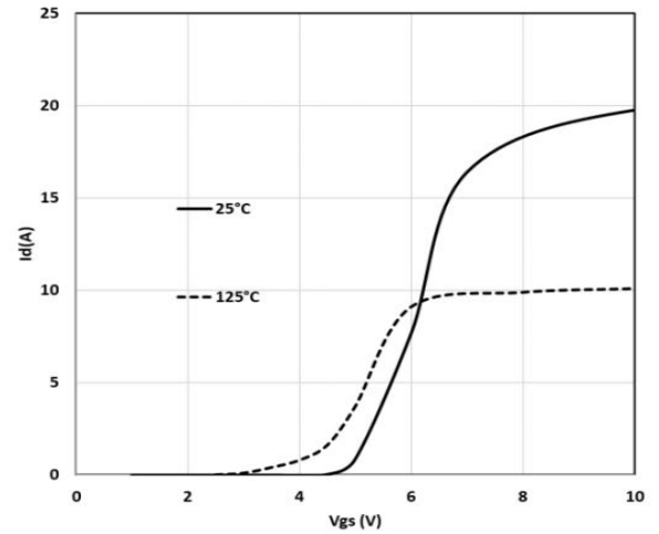
Fig.2 Transfer characteristics
