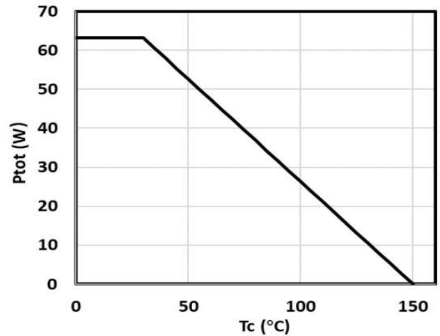
Fig.4 Power dissipation
