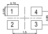
SUGGEST LAYOUT
