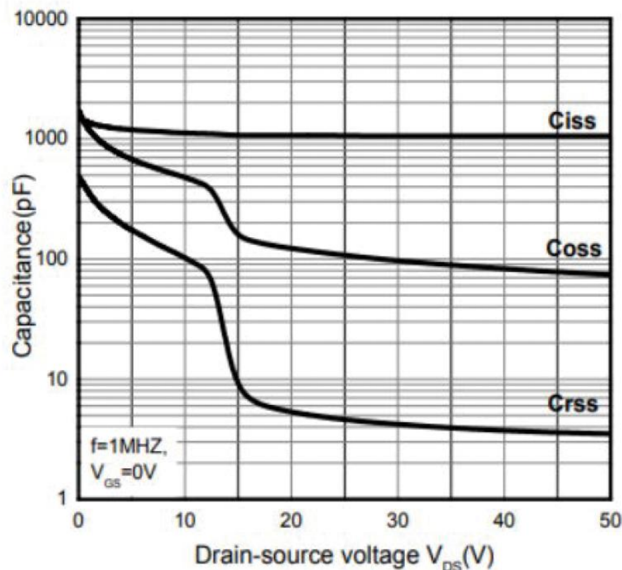
Figure.3 Capacitance Characteristics
