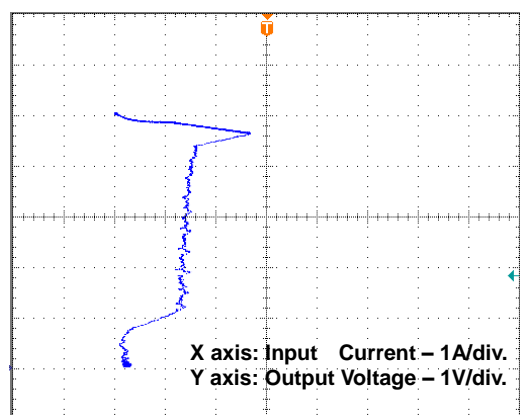
Figure 15. Over Current Protection Characteristics
