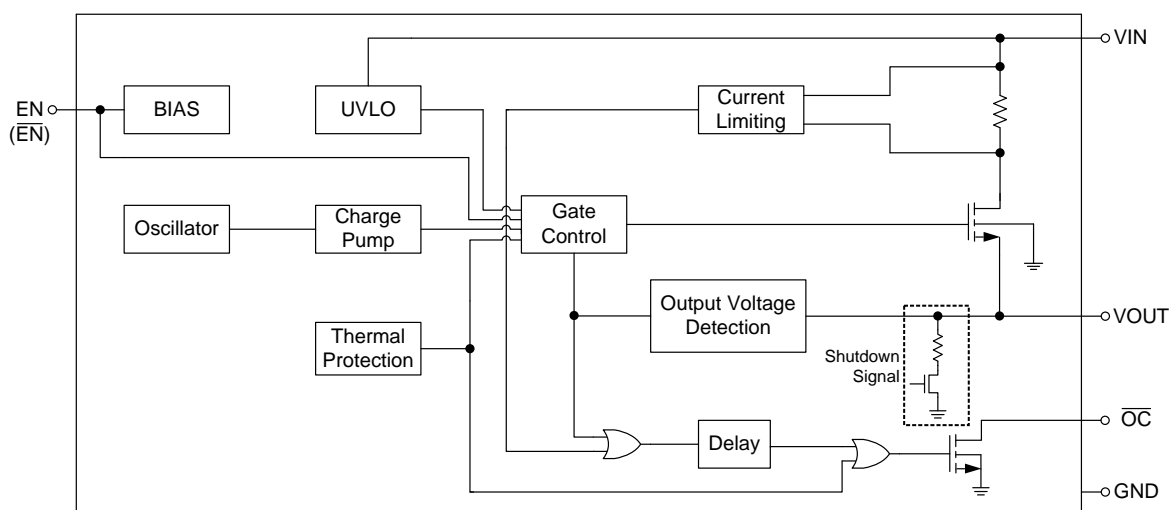
Figure 3. Block Diagram
