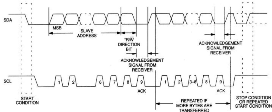
DATA TRANSFER ON 2-WIRE SERIAL BUS Figure 5
