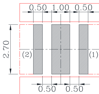
Recommended Solder Pad
